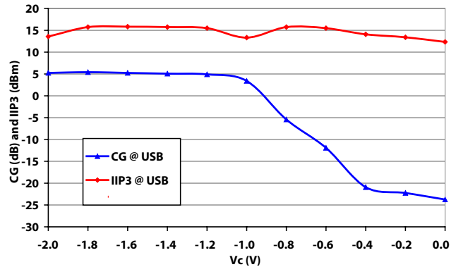
USB Conversion Gain Vs Control Voltage (Vc), 36GHz Vg2=-0.5V, Vd=4V, Id=240mA, P_LO=+4dBm
