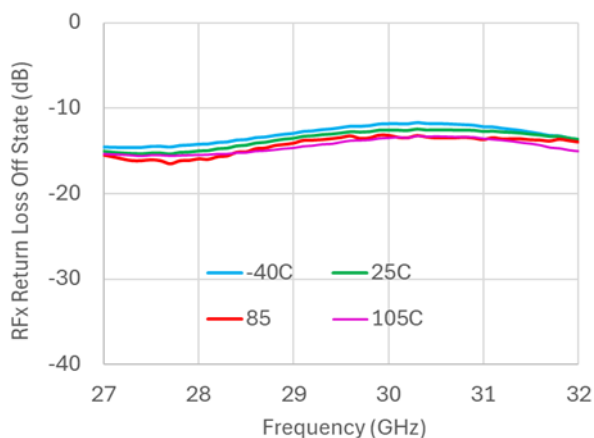
Return Loss: RF1/RF2 (Off State)
