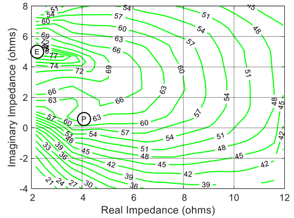
P2.5dB Loadpull AM/PM Contours (°)
