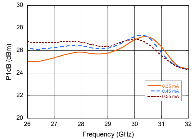
P1dB vs. Frequency over Bias Voltage
