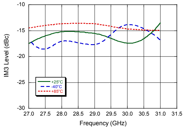
IM3 over Temperature ( P_{OUT} = 30\text{ dBm / Tone} )
