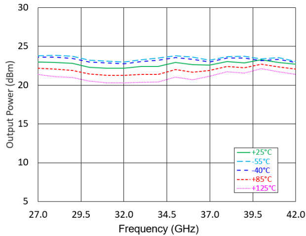
Output Power vs. Frequency @ P_{IN} = 1 dBm
