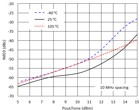
IMD3 vs. Output power / tone, 1.8 GHz
