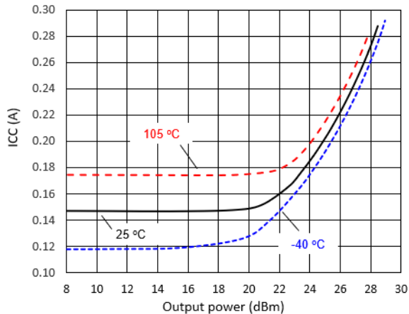
ICC vs. Output power 11 , 2.5 GHz
