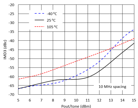
IMD3 vs. Output power / tone, 2.5 GHz
