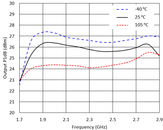
Output P_{1dB}^{11} , 1.7 - 2.9 GHz
