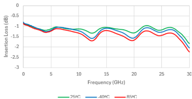
Insertion Loss
