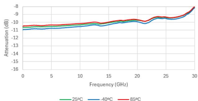
Attenuation (Normalized)
