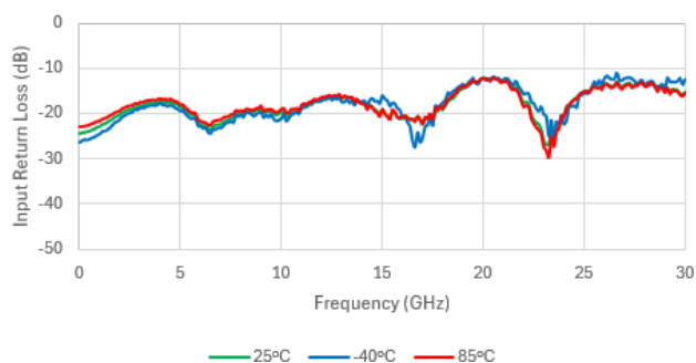
Input Return Loss (Insertion Loss State)
