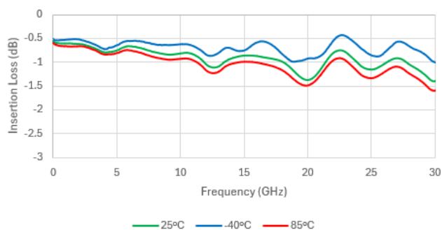
Insertion Loss
