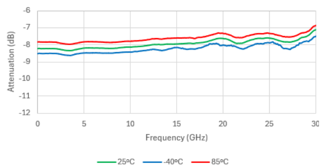
Attenuation (Normalized)
