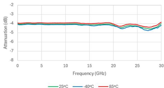
Attenuation (Normalized)
