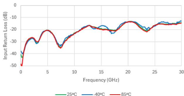
Input Return Loss (Attenuation State)
