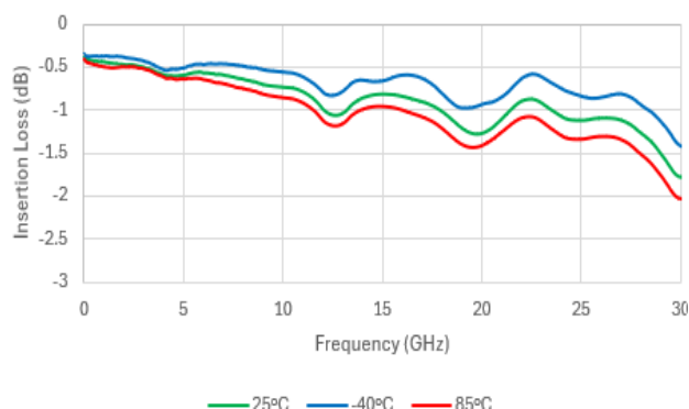
Insertion Loss
