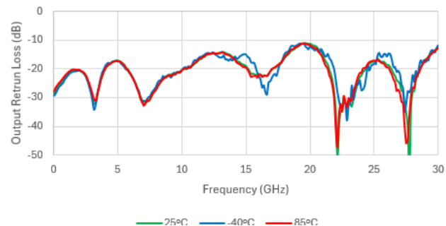
Output Return Loss (Attenuation State)
