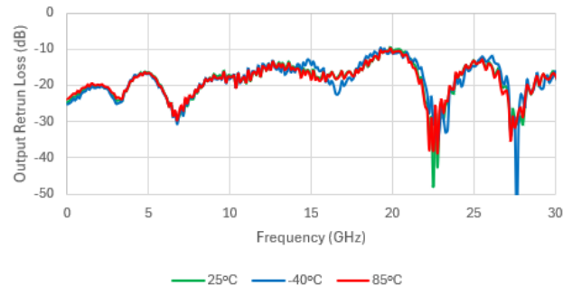
Output Return Loss (Insertion Loss State)
