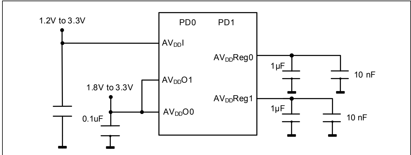
Figure 4-3. Supply configuration, both channels and both A and B outputs used
