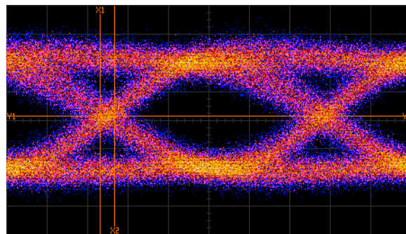
Unfiltered Eye Diagram for 2.5 Gbps @ -26 dBm
