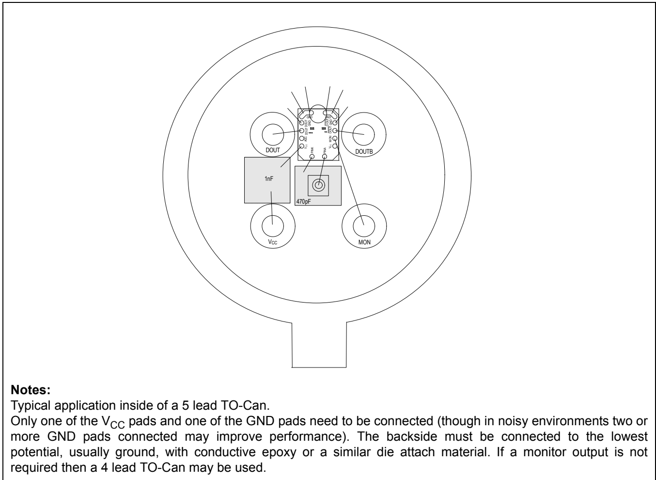
Figure 4-2. Typical Layout Diagram with Photodiode Mounted on PINK Capacitor (5 pin TO-Can)
